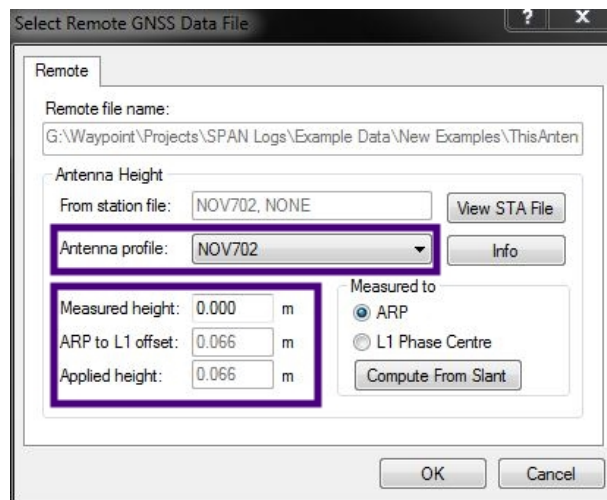
Figure 4: When adding a remote or base station file, the Antenna Profile will be auto-filled using information from the THISANTENNATYPEEB log, read in from the STA file
